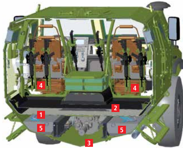
■ Vehicle section: (1) floor, (2) suspended floor, (3) V-shield, (4) anti-mine seats with side and ceiling fixtures, (5) independent fuel tanks
