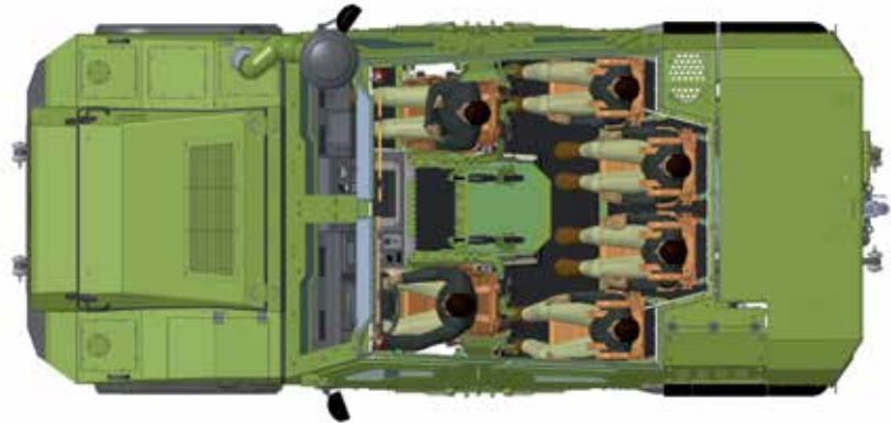
■ Layout of the 6-member crew in the Gerlach safety capsule
